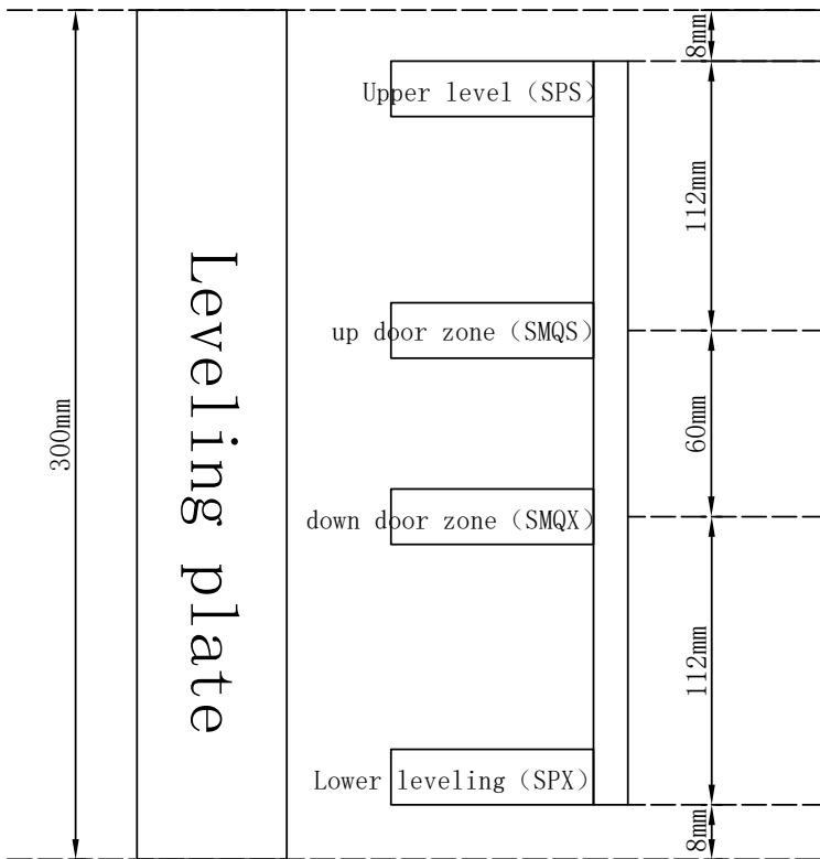
Installation of leveling switches
