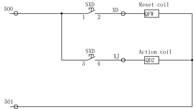
MRL Overspeed governor mechanical action and reset circuit
