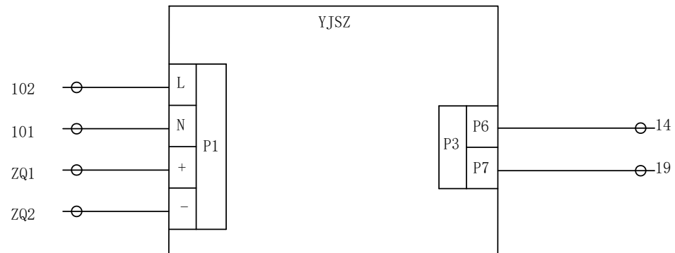
Emergency brake release device circuit(Double door)
