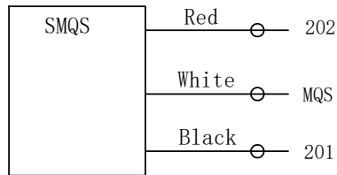
Leveling switches type: SGD31-GG-TZ2B2
