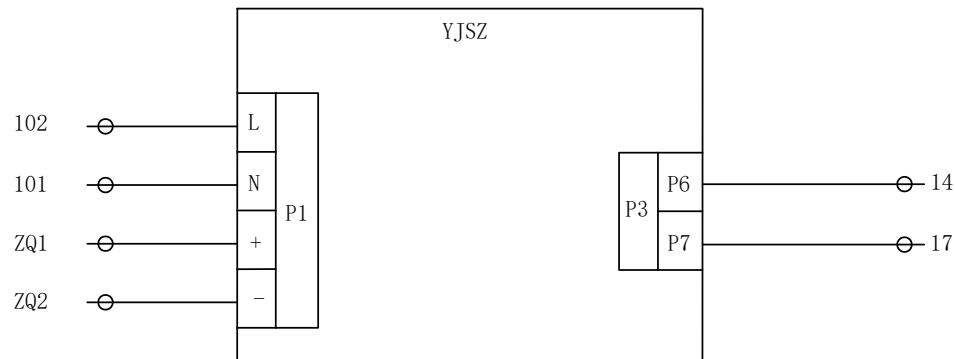
Emergency brake release device circuit(single door)
